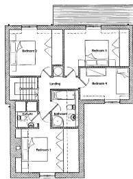
Proposed First Floor Layout
