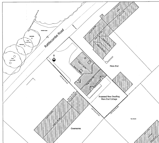
Proposed Blockplan scale 1:200
